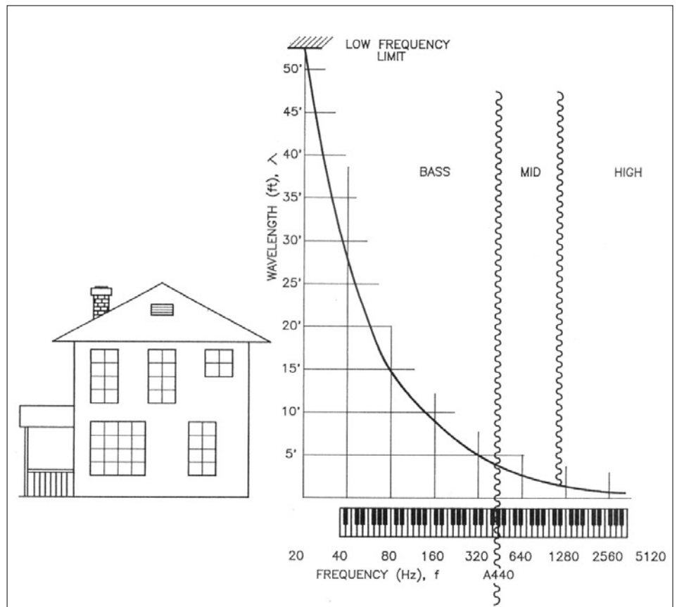
Figure 2. Wavelengths of sound.
