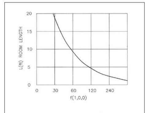
Figure 11. Lowest resonance frequency.
