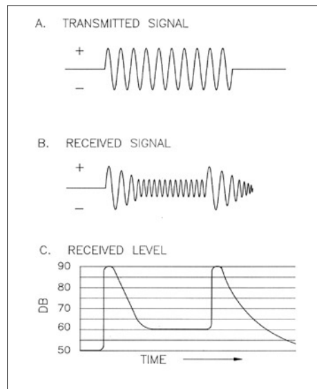
Figure 14. Burst in a room (middle).
