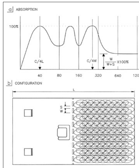
Figure 5. Traps with backscattering.
