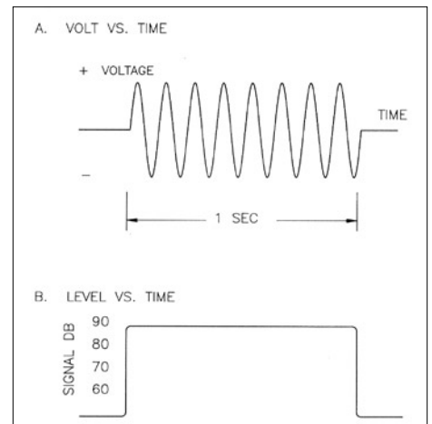
Figure 12. The tone burst.
