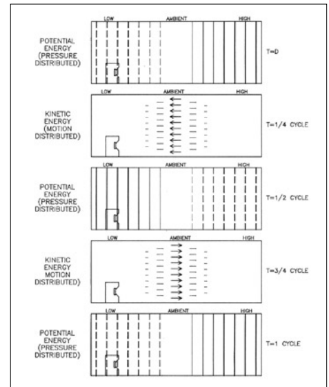
Figure 7. 1st room resonance (1,0,0).
