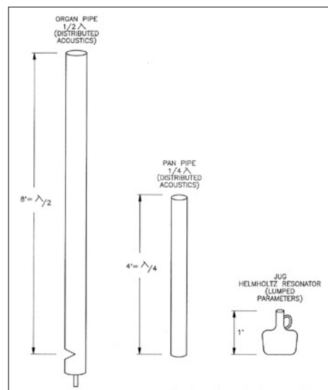
Figure 8. Lumped and distributed parameters.
