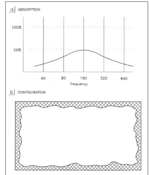
Figure 6. membrane traps.
