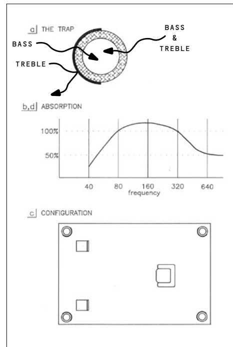
Figure 12. The “functional” trap.
