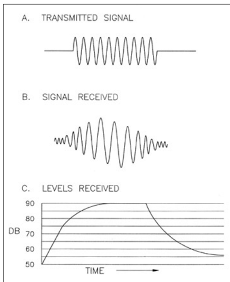
Figure 13. Burst in a room (end).
