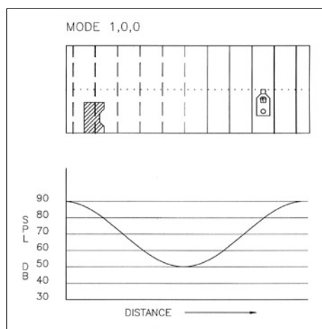
Figure 10. Sound level distribution.
