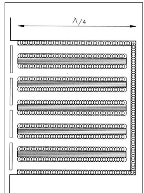
Figure 9. A classic \frac{1}{4} \lambda trap.
