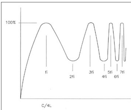
Figure 3. 1/4 lambda trap response.
