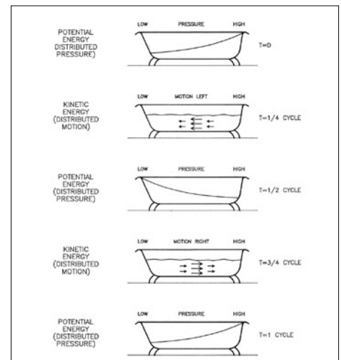
Figure 8. Bathtub mode (1,0,0).
