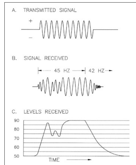
Figure 15. Resonance coloration.
