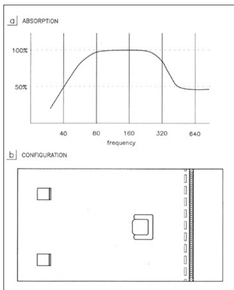
Figure 7. Pressure zone trap.
