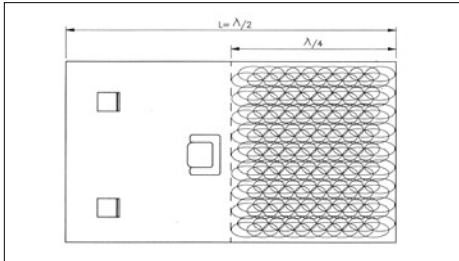
Figure 2. 1/4 wavelength trap.
